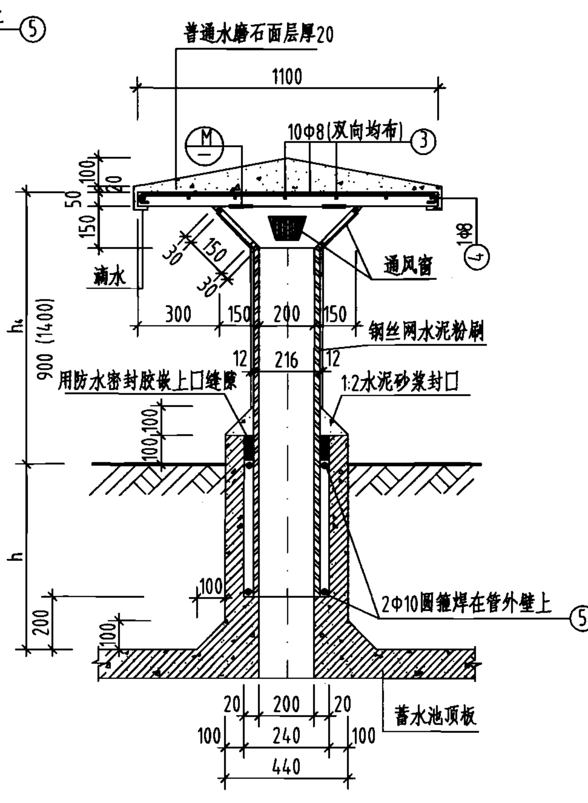
2-2
